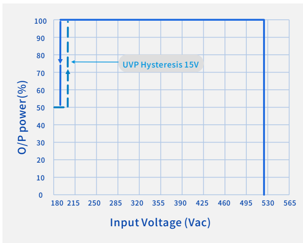
O/P Power Vs. Input Voltage
